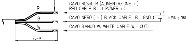
ELECTRIC WIRING MOTOR DIAGRAM
