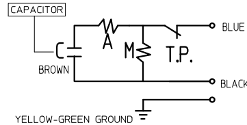
ELECTRIC WIRING MOTOR DIAGRAM
